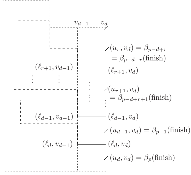
FIGURE 3. Partitioning the maximal faces of \mathcal{C}_u^v into S_{\underline{\ell}}
