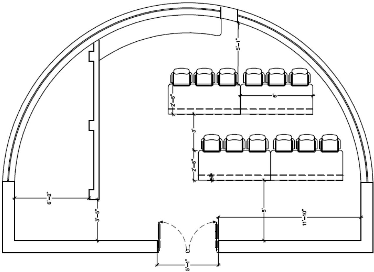
Schematic diagram of the Media Room
