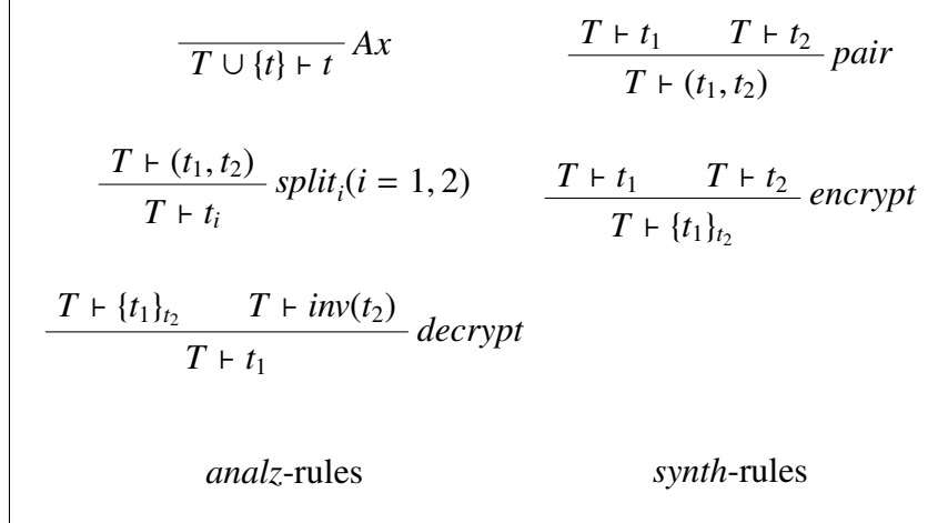
Fig. 1. Message generation rules.
