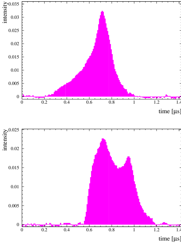
Fig. 6 Top: Shape of one candidate for 0\nu\beta\beta decay classified as SSE by all three methods of pulse shape discrimination. Bottom: Shape of one candidate classified as MSE by all three methods.
