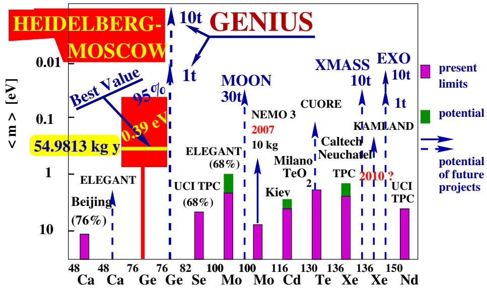
Fig. 19 Present evidence for 0\nu\beta\beta decay from data of the HEIDELBERG-MOSCOW experiment and the potential of present and future \beta\beta experiments. Vertical axis - effective neutrino mass limits (only HEIDELBERG-MOSCOW gives a value) in eV, horizontal - isotopes used in the various experiments.
