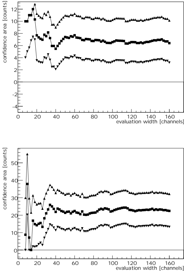
Fig. 9 Top : Analysis of simulated spectrum with Gaussian peak of 5 events and FWHM of 9.4 channels on a Poisson-distributed background spectrum of 0.5 events/channel, as function of interval of analysis. The middle line is the best value. Upper and lower lines correspond to the 68.3% confidence limits. Bottom : The same as above, but the peak contains 20 events, the background is 4 events/channel. One channel corresponds to 0.36 keV in our measured spectra.
