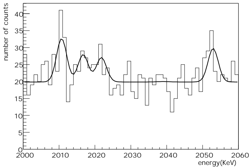
Fig. 17 Analysis of the spectrum measured by D. Caldwell et al. 92 , with the Maximum Likelihood Method, in the energy range 2000 - 2060 keV (as in Fig.13) assuming lines at 2010.78, 2016.70, 2021.60, 2052.94, 2039.0 keV. In contrast to Fig.13 no indication for a signal at 2039 keV is observed (see text).
