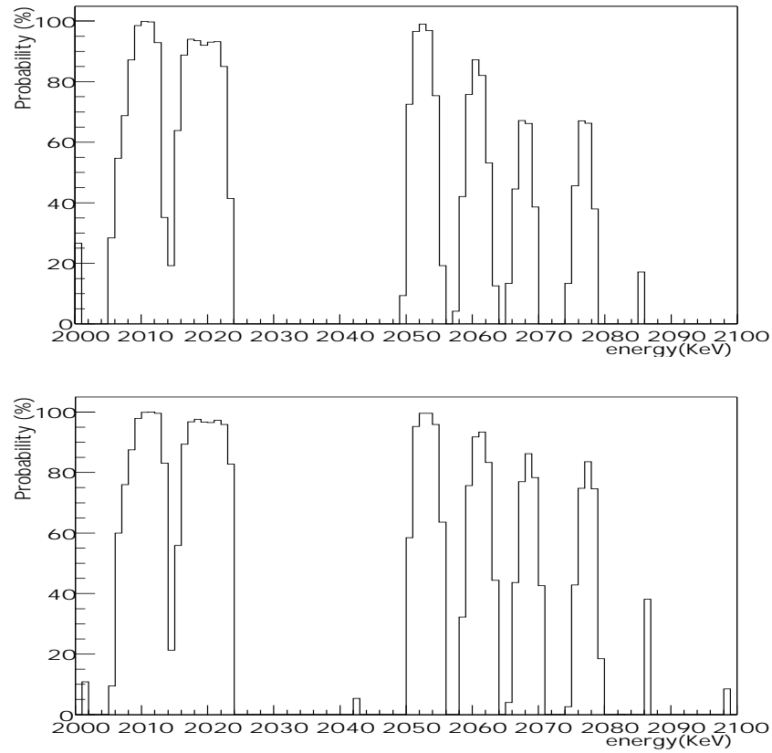
Fig. 16 Peak scanning of the spectrum measured by Caldwell et al. 92 with the Maximum Likelihood method (upper part), and with the Bayesian method (lower part) (as in Fig.10,11,12) (see ref.[74]).
