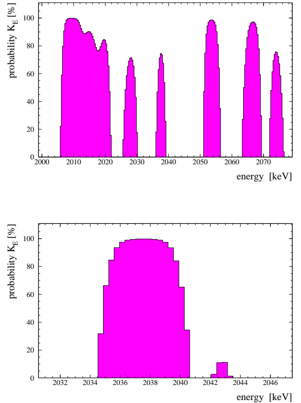
Fig. 11 Top: Probability K_E that a line exists at a given energy in the range of 2000-2080 keV derived via Bayesian inference from the spectrum taken with detectors Nr. 1,2,3,5 over the period August 1990 to May 2000, 46.502 kg y (see Fig.2 from ref.[43]). Bottom: Result of a Bayesian scan for lines as in the left part of this figure, but in the energy range of analysis \pm 5\sigma around Q_{\beta\beta} .
