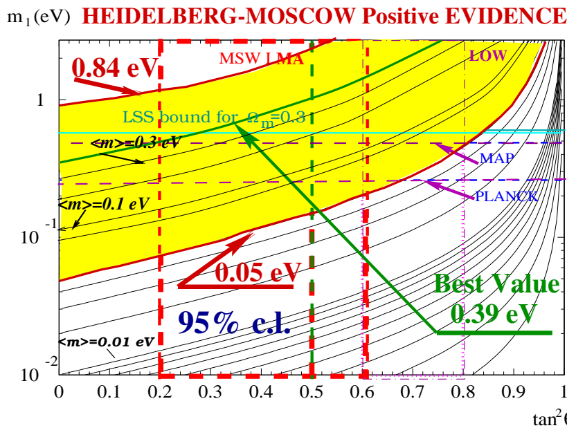
Fig. 21 Double beta decay observable \langle m \rangle and oscillation parameters: The case for degenerate neutrinos. Plotted on the axes are the overall scale of neutrino masses m_0 and mixing \tan^2 \theta_{12} . Also shown is a cosmological bound deduced from a fit of CMB and large scale structure 112 and the expected sensitivity of the satellite experiments MAP and PLANCK. The present limit from tritium \beta decay of 2.2 eV 113 would lie near the top of the figure. The range of \langle m \rangle fixed by the HEIDELBERG-MOSCOW experiment is, in the case of small solar neutrino mixing, already in the range to be explored by MAP and PLANCK.
