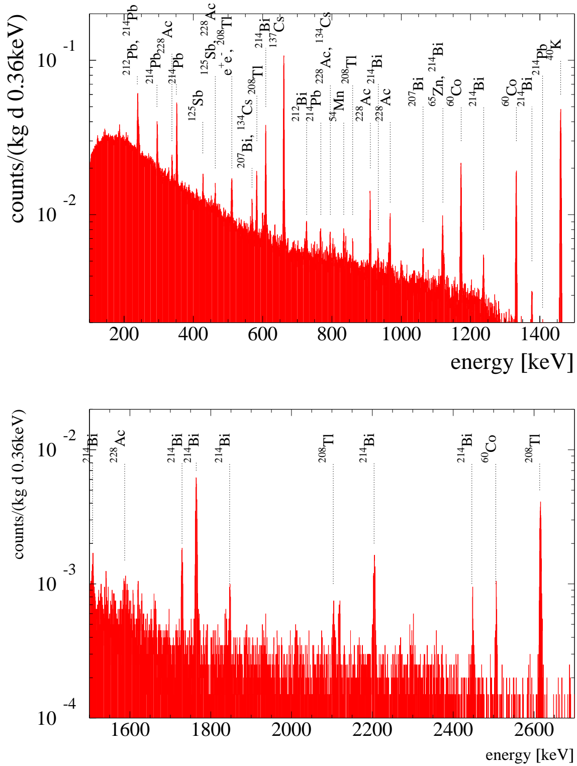
Fig. 3 Sum spectrum of enriched detectors Nr. 1,2,3,4,5 over the period August 1990 - May 2000 (54.9813 kg y) measured in the HEIDELBERG-MOSCOW experiment (binning 0.36 keV). The sources of the main identified background lines are noted.
