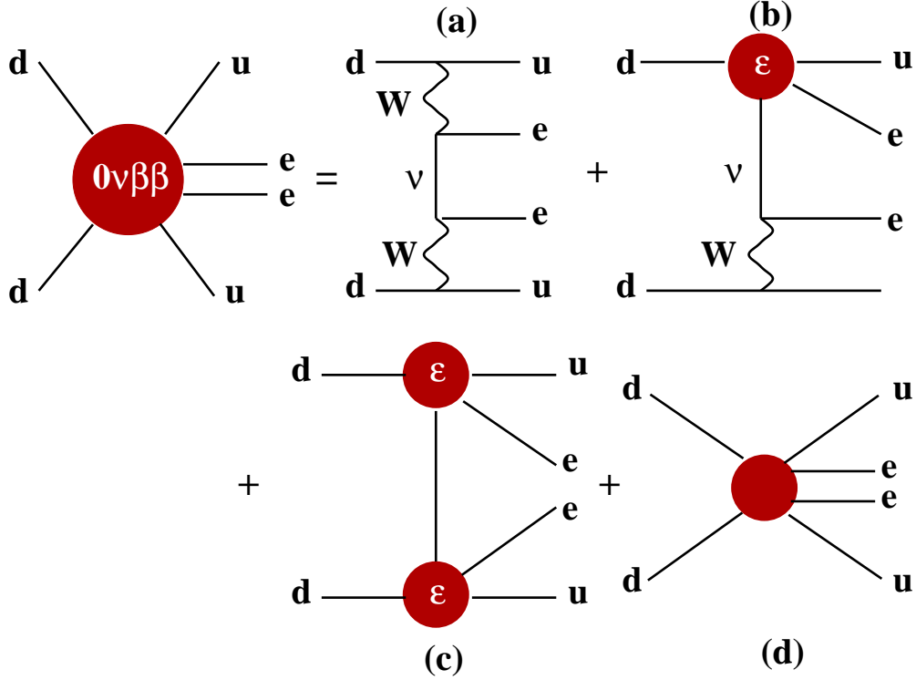
Fig. 1 Feynman graphs of the general double beta decay with long range (a-c) and short range (d) parts (see ref.[18]).
