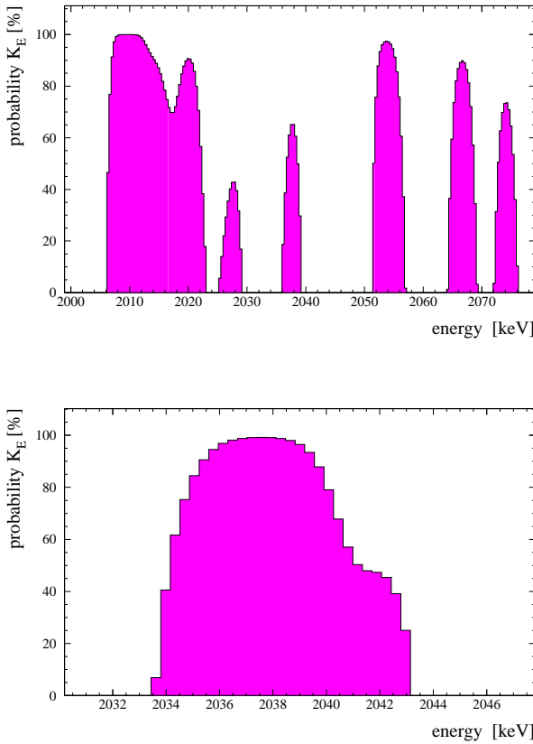
Fig. 10 Scan for lines in the full spectrum taken from 1990-2000 with detectors Nr. 1,2,3,4,5, (Fig.4), with the Bayesian method of sec. 3.1. The ordinate is the probability K_E that a line exists as defined in the text. Top: Energy range 2000 - 2080 keV. Bottom: Energy range of analysis \pm 5\sigma around Q_{\beta\beta} .
