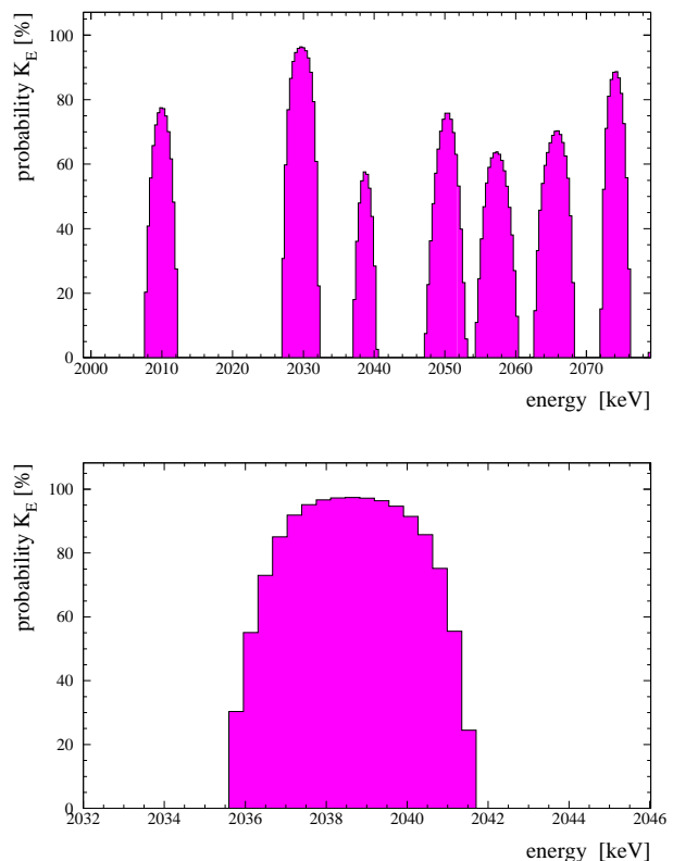
Fig. 12 Scan for lines in the single site event spectrum taken from 1995-2000 with detectors Nr. 2,3,5, (Fig.5), with the Bayesian method (as in Figs.10,11). Top: Energy range 2000 -2080 keV. Bottom: Energy range of analysis \pm 4.4\sigma around Q_{\beta\beta} .
