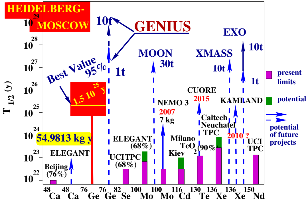
Fig. 18 Present evidence for 0\nu\beta\beta decay from data of the HEIDELBERG-MOSCOW experiment and the potential of present and future \beta\beta experiments. Vertical axis - half life limits (only HEIDELBERG-MOSCOW gives a value) in years, horizontal - isotopes used in the various experiments.
