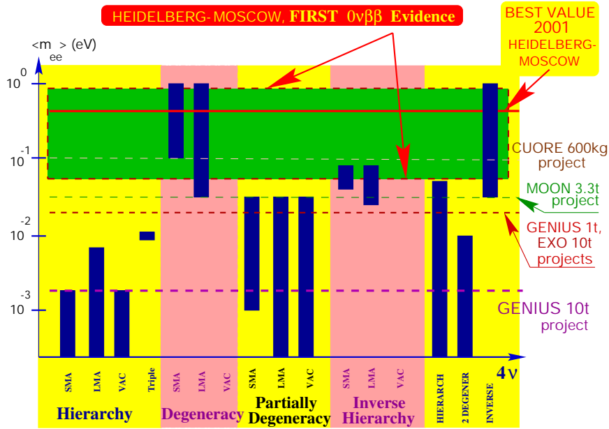
Fig. 20 The impact of the evidence obtained for neutrinoless double beta decay in this paper (best value of the effective neutrino mass \langle m \rangle = 0.39 eV, 95% confidence range (0.05 - 0.84) eV - allowing already for an uncertainty of the nuclear matrix element of a factor of \pm 50\% ) on possible neutrino mass schemes. The bars denote allowed ranges of \langle m \rangle in different neutrino mass scenarios, still allowed by neutrino oscillation experiments. Hierarchical models are excluded by the new 0\nu\beta\beta decay result. Also shown are the expected sensitivities for the future potential double beta experiments CUORE, MOON, EXO and the 1 ton and 10 ton project of GENIUS 98 (from ref.[5]).
