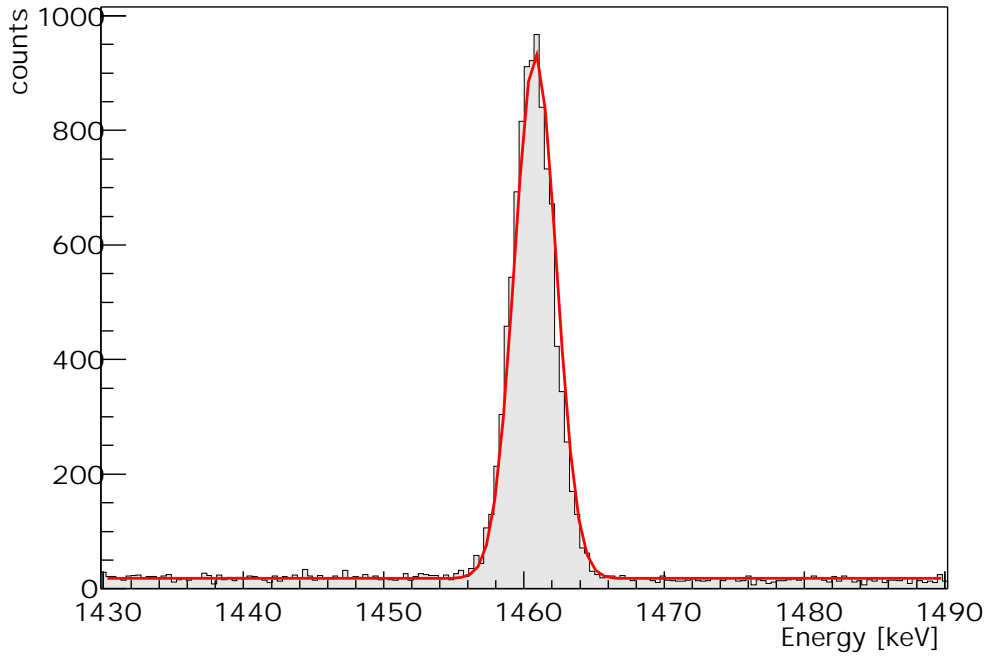
Fig. 7 Fit of one the lines (here the 1460.81 keV line from ^{40}\text{K} ) in the sum spectrum of all five detectors, used for the calibration and the determination of the energy resolution (see Table IV).
