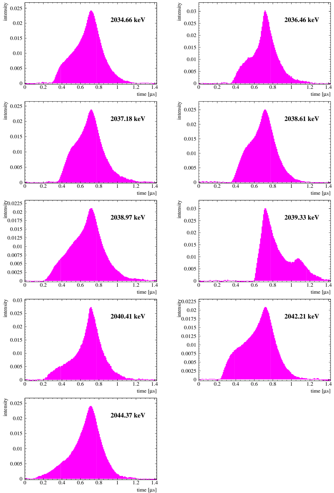
Fig. 14 Events classified to be single site events (SSE) by all three methods of PSA in the range 2034.1 - 2044.9 keV, in the measurement period 10.1995 - 05.2000, 28.053 kg y.
