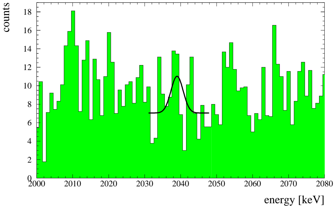
Fig. 4 Sum spectrum of the ^{76}\text{Ge} detectors Nr. 1,2,3,4,5 over the period August 1990 to May 2000, (54.9813 kg y) in the energy interval 2000 - 2080 keV, around the Q_{\beta\beta} value of double beta decay ( Q_{\beta\beta} = 2039.006(50) keV) summed to 1 keV bins. The curve results from Bayesian inference in the way explained in sec.3. It corresponds to a half-life T_{1/2}^{0\nu} = (0.80 - 35.07) \times 10^{25} y (95% c.l.)
