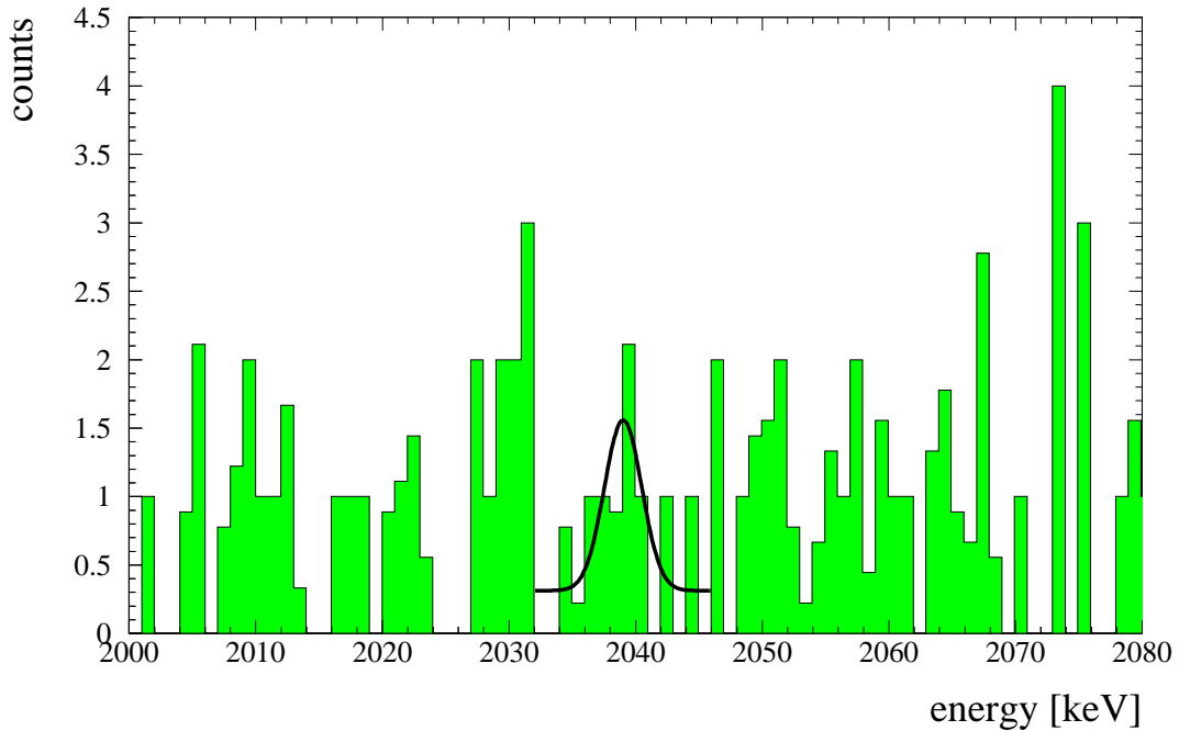
Fig. 5 Sum spectrum of single site events, measured with the detectors Nr. 2,3,5 operated with pulse shape analysis in the period November 1995 to May 2000 (28.053 kg y), summed to 1 keV bins. Only events identified as single site events (SSE) by all three pulse shape analysis methods 84-86 have been accepted. The curve results from Bayesian inference in the way explained in sec.3. When corrected for the efficiency of SSE identification (see text), this leads to the following value for the half-life: T_{1/2}^{0\nu} = (0.88 - 22.38) \times 10^{25} y (90% c.l.).
