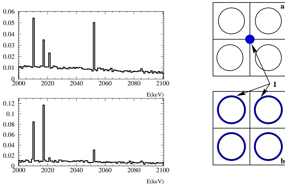
Fig. 8 Demonstration of the dependence of the relative intensities of the weak ^{214}\text{Bi} lines on the location of the impurity in the experimental setup. The right side shows two different locations of the impurity (1) relative to the detectors. The left side shows the corresponding different relative intensities to be expected. Top : Source in some distance from the detectors (as in a) (right part). Bottom : Source in copper cap very near around the detectors (as in b) (right part). The ordinate shows relative intensities (see ref.[44]).
