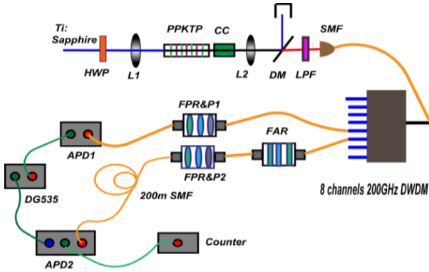
Figure 1. The layout of the experiment.
