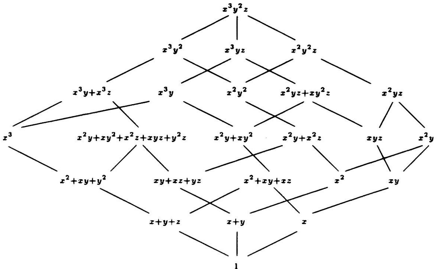
FIGURE 14. Simple Schubert polynomials for S_4
