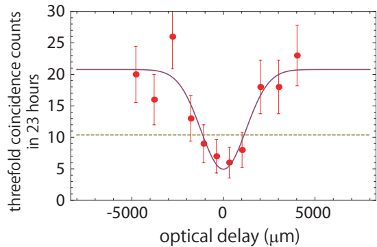
Figure 2: Observed HOM interference between two light pulses. The threefold coincidence counts have been observed in the 300-ps time windows. Solid curves are Gaussian fitted to the experimental counts. Dashed horizontal lines describe the minimum values of the dips in the classical wave theory.
