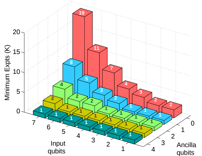
Figure 1: Minimum number of independent experiments required for QST (with zero ancilla) and AAQST.
