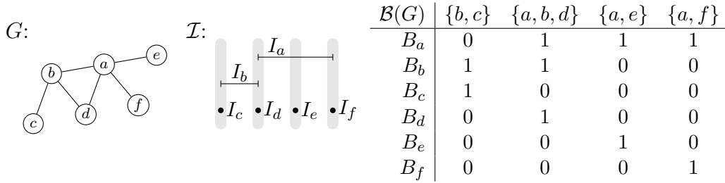
Figure 1: An interval graph G , a minimal interval model \mathcal{I} of G , and the bundle hypergraph \mathcal{B}(G) of G . The latter is given by its incidence matrix with columns indexed by vertices (i.e., maxcliques) and rows indexed by hyperedges (i.e., bundles).
