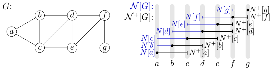
Figure 5: From an interval ordering of \mathcal{N}[G] to a tight interval model \mathcal{N}^+[G] of G .
